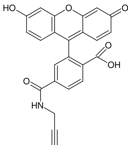
Structural formula of 6-FAM-Alkyne
