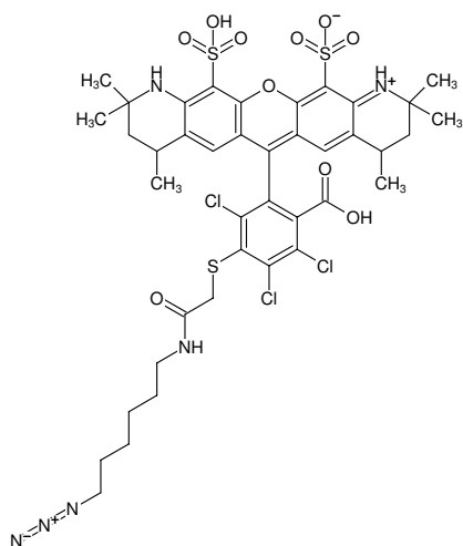
Structural formula of AF546-Azide
