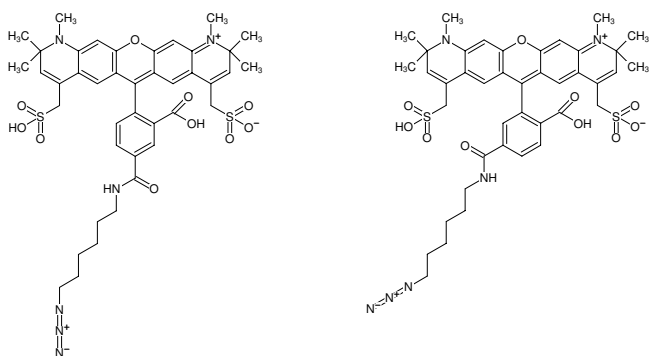
Structural formula of AF594-Azide
