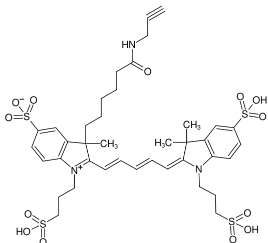
Structural formula of AF647-Alkyne
