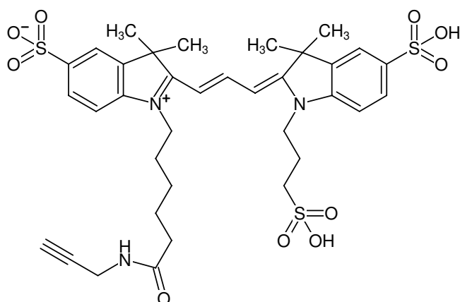
Structural formula of Sulfo-Cy3-Alkyne
