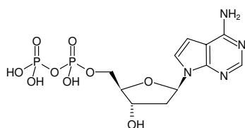
Structural formula of 7-Deaza-dADP
