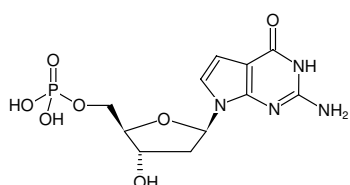
Structural formula of 7-Deaza-dGMP
