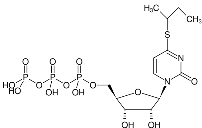
Structural formula of 4-Thio- i -butyl-UTP
