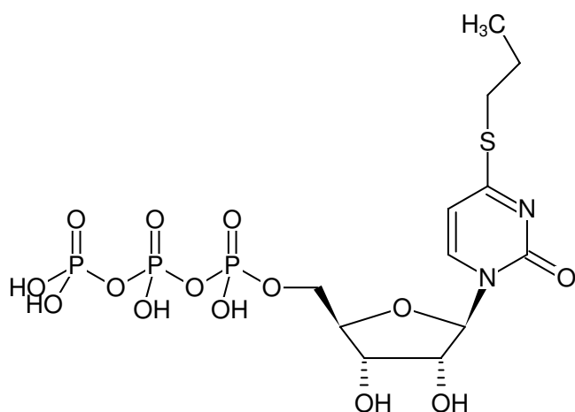
Structural formula of 4-Thio- n -propyl-UTP
