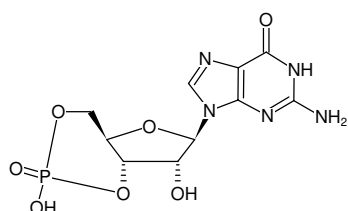
Structural formula of cGMP
