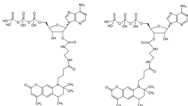
Structural formula of EDA-ATPyS-ATTO-390
