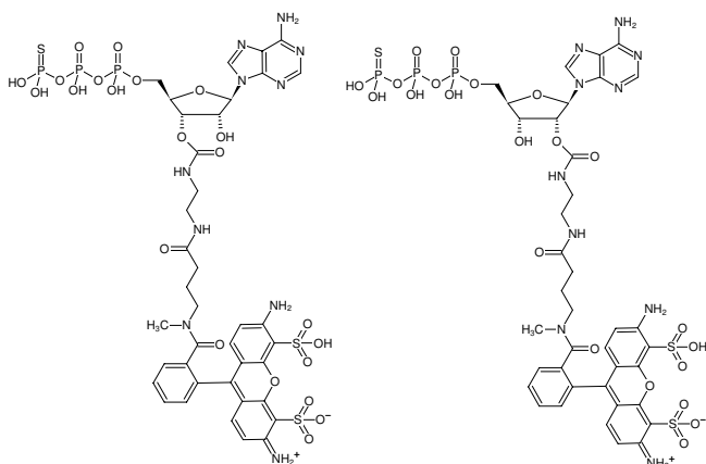
Structural formula of EDA-ATPyS-ATTO-488
