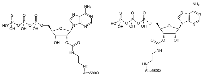
Structural formula of EDA-ATPyS-ATTO-580Q
