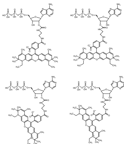
Structural formula of EDA-ATPyS-ATTO-590
