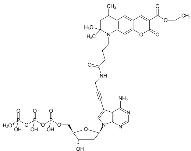
Structural formula of 7-Propargylamino-7-deaza-dATP-ATTO-425
