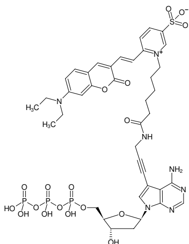
Structural formula of 7-Propargylamino-7-deaza-dATP-DY-480XL
