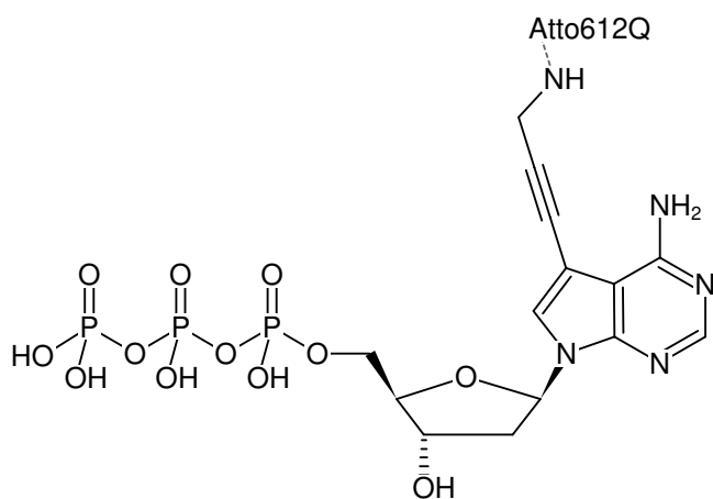
Structural formula of 7-Propargylamino-7-deaza-dATP-ATTO-612Q
