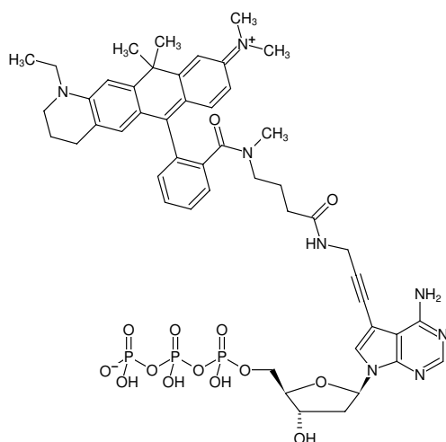
Structural formula of 7-Propargylamino-7-deaza-dATP-ATTO-633
