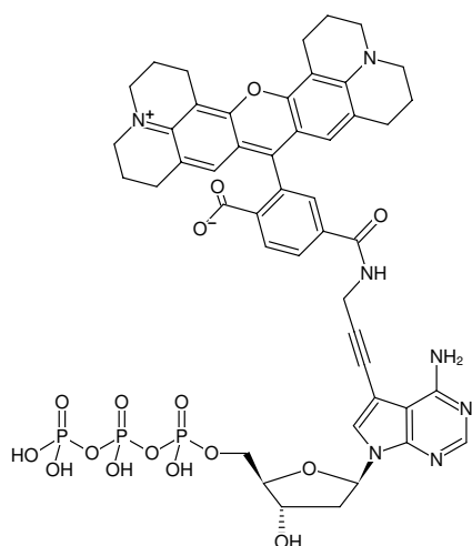
Structural formula of 7-Propargylamino-7-deaza-dATP-6-ROX
