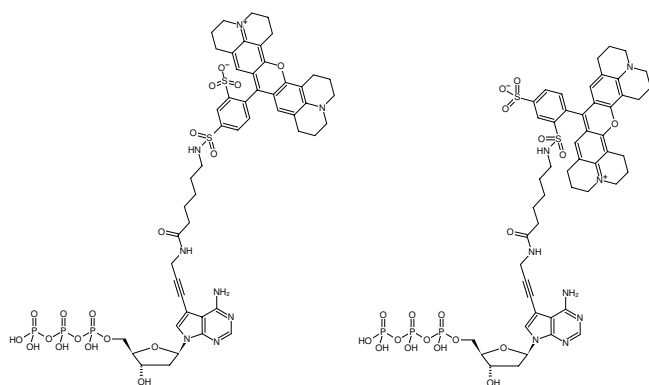
Structural formula of 7-Propargylamino-7-deaza-dATP-Texas Red
