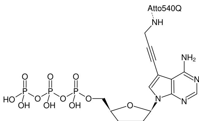
Structural formula of 7-Propargylamino-7-deaza-ddATP-ATTO-540Q
