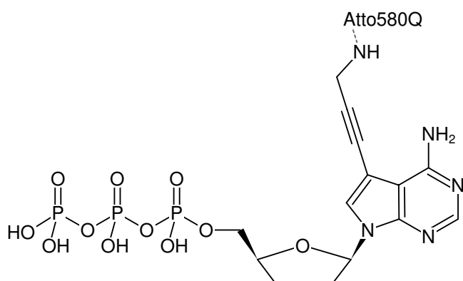
Structural formula of 7-Propargylamino-7-deaza-ddATP-ATTO-580Q
