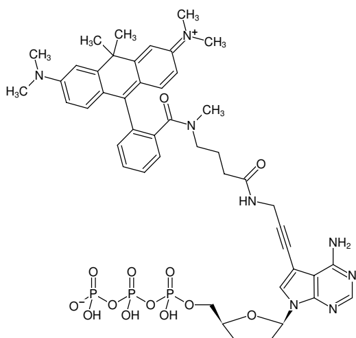
Structural formula of 7-Propargylamino-7-deaza-ddATP-ATTO-620
