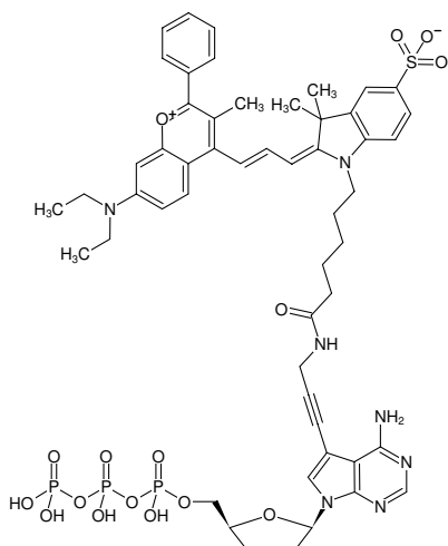
Structural formula of 7-Propargylamino-7-deaza-ddATP-DYQ-660
