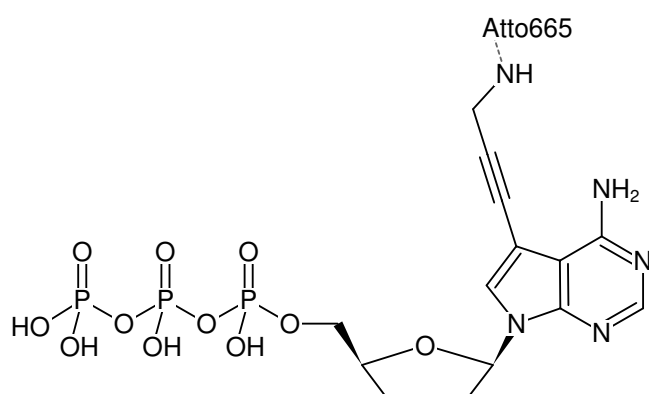
Structural formula of 7-Propargylamino-7-deaza-ddATP-ATTO-665
