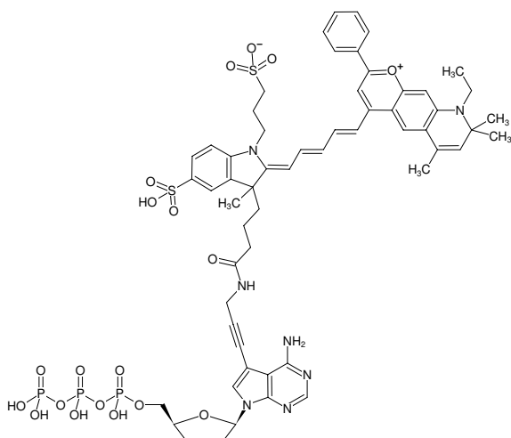
Structural formula of 7-Propargylamino-7-deaza-ddATP-DY-776
