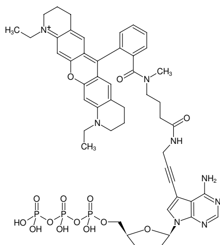
Structural formula of 7-Propargylamino-7-deaza-ddATP-ATTO-Rho11
