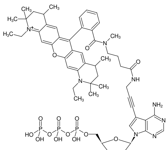
Structural formula of 7-Propargylamino-7-deaza-ddATP-ATTO-Rho12
