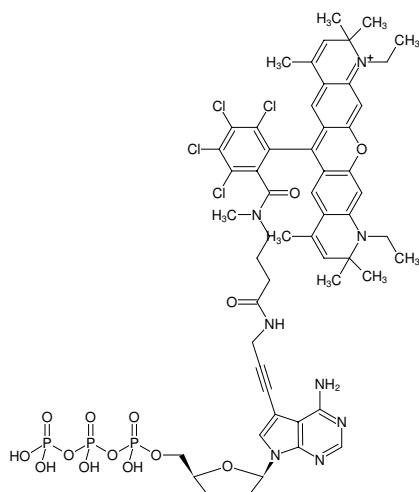
Structural formula of 7-Propargylamino-7-deaza-ddATP-ATTO-Rho14
