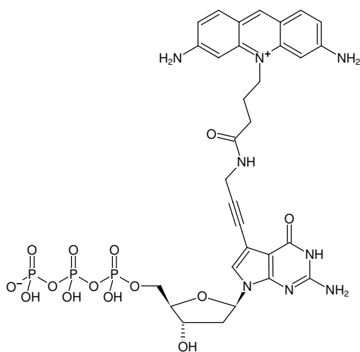
Structural formula of 7-Propargylamino-7-deaza-dGTP-ATTO-465
