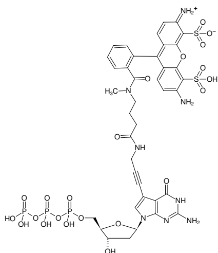
Structural formula of 7-Propargylamino-7-deaza-dGTP-ATTO-488
