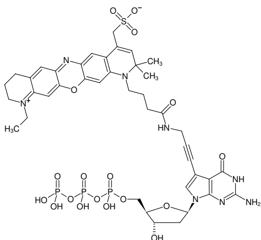
Structural formula of 7-Propargylamino-7-deaza-dGTP-ATTO-680
