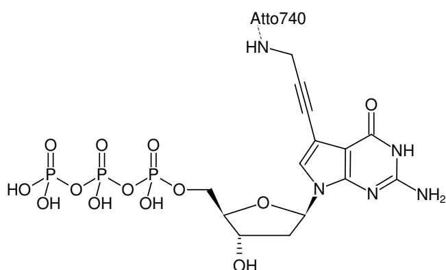
Structural formula of 7-Propargylamino-7-deaza-dGTP-ATTO-740
