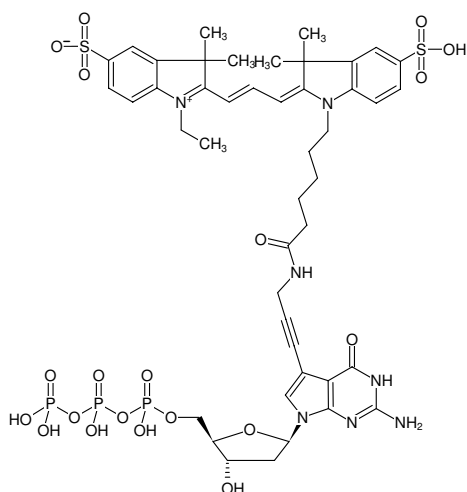
Structural formula of 7-Propargylamino-7-deaza-dGTP-Cy3
