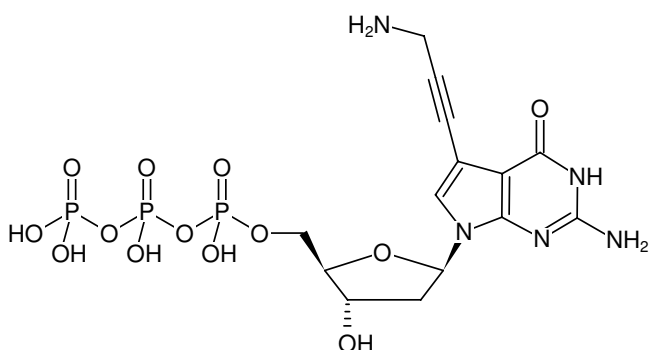
Structural formula of 7-Deaza-7-propargylamino-dGTP
