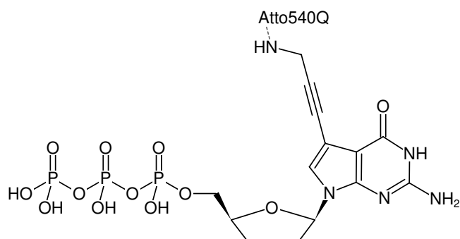
Structural formula of 7-Propargylamino-7-deaza-ddGTP-ATTO-540Q
