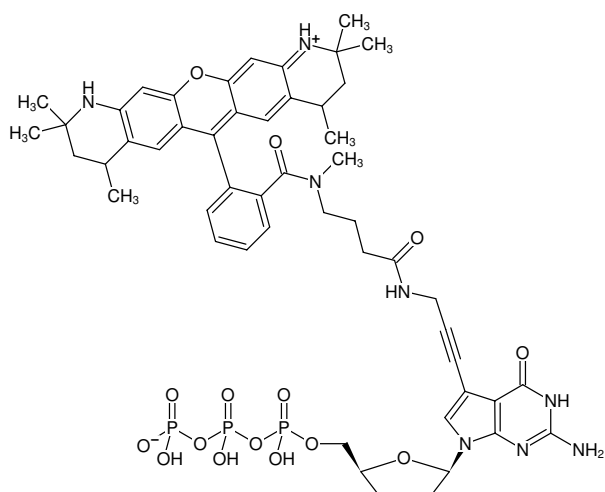
Structural formula of 7-Propargylamino-7-deaza-ddGTP-ATTO-550
