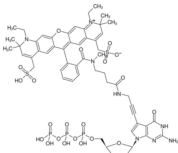
Structural formula of 7-Propargylamino-7-deaza-ddGTP-ATTO-594
