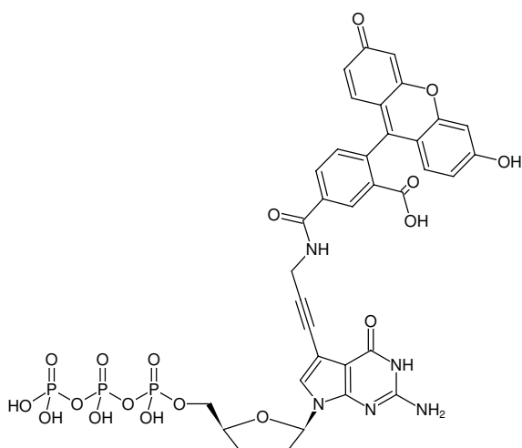
Structural formula of 7-Propargylamino-7-deaza-ddGTP-5-FAM
