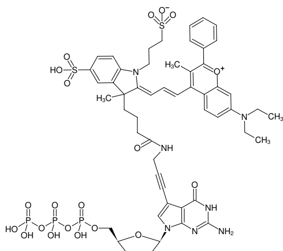
Structural formula of 7-Propargylamino-7-deaza-ddGTP-DYQ-661
