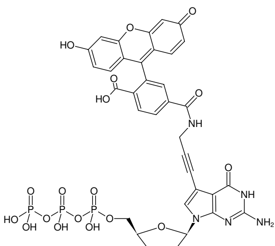
Structural formula of 7-Propargylamino-7-deaza-ddGTP-6-FAM
