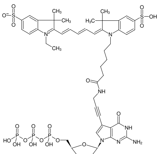
Structural formula of 7-Propargylamino-7-deaza-ddGTP-Cy5
