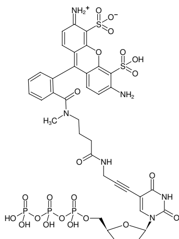
Structural formula of 5-Propargylamino-ddUTP-ATTO-488
