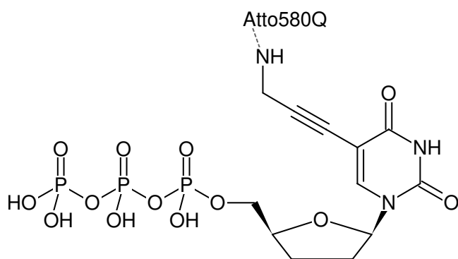
Structural formula of 5-Propargylamino-ddUTP-ATTO-580Q
