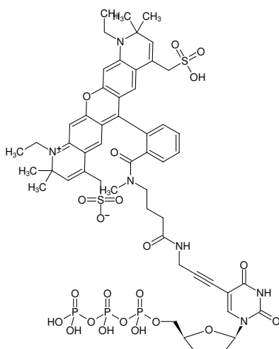
Structural formula of 5-Propargylamino-ddUTP-ATTO-594
