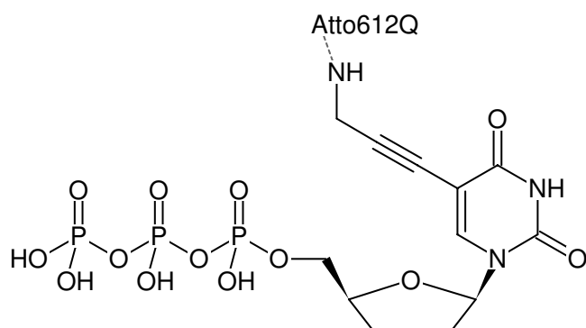
Structural formula of 5-Propargylamino-ddUTP-ATTO-612Q
