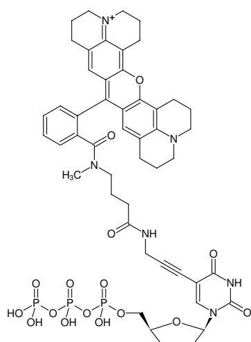
Structural formula of 5-Propargylamino-ddUTP-ATTO-Rho101
