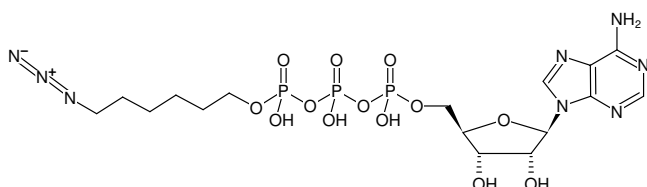
Structural formula of \gamma -(6-Azidoheptyl)-ATP
