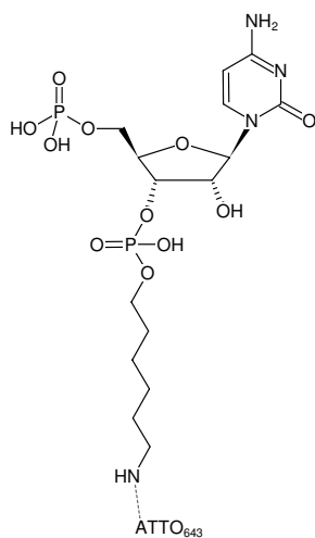
Structural formula of pCp-ATTO-643
