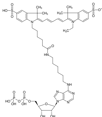
Structural formula of N 6 -(6-Aminoethyl)-ADP-Cy5
